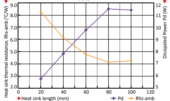
ModuLED Pico performance data at a heat sink to ambient temperature difference, \Delta T_{hs-amb} , of 50 °C
