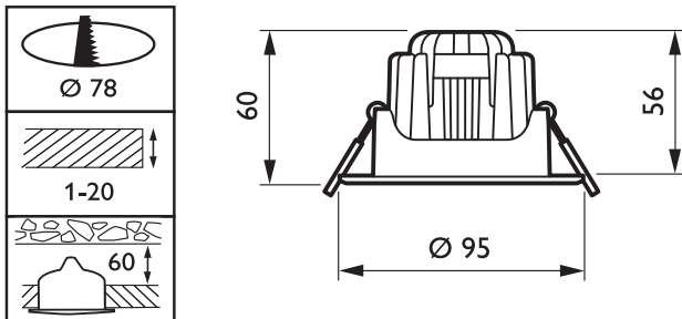
RS140B LED6-32-/840 PSR PI6 WH
