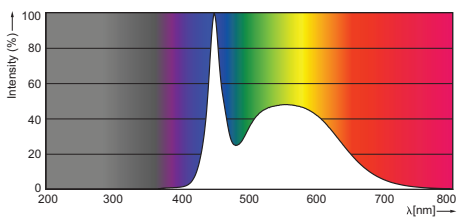
LED tube 1500 mm 22 W /865 C
